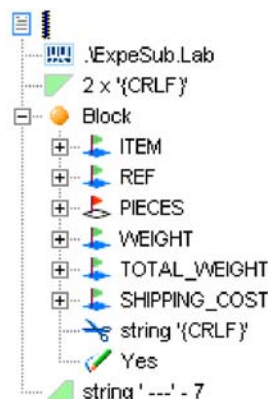
Figure 16 The tree displays the structure
